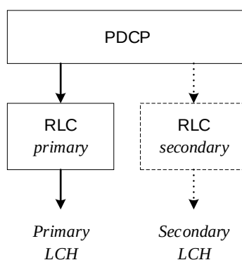
Figure 16.1.3-1: Packet Duplication
